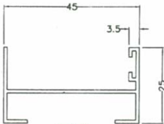
SD144 0.329 kg/m AP:233 mm
