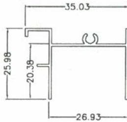
SW078 0.280 kg/m AP: 199 mm
