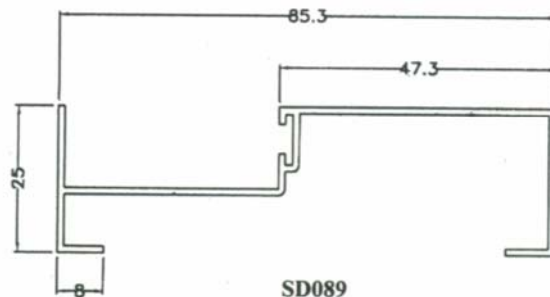
SD089 0.512 kg/m AP:337 mm
