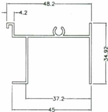
SD399 0.391 kg/m AP:273 mm
