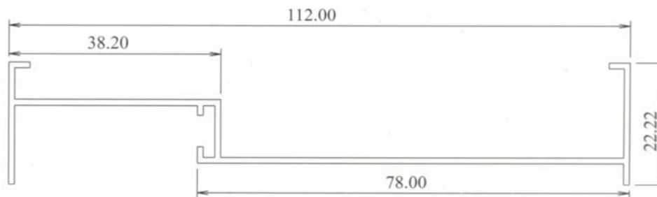
SD170N 0.533 kg/m AP: 361 mm
