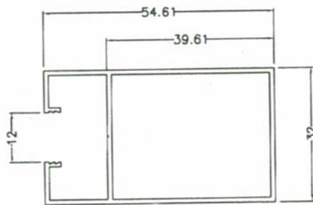
SD095 0.578 kg/m AP:252 mm
