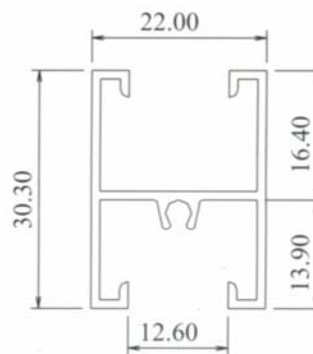
SD9819 0.342 kg/m AP: 222 mm
