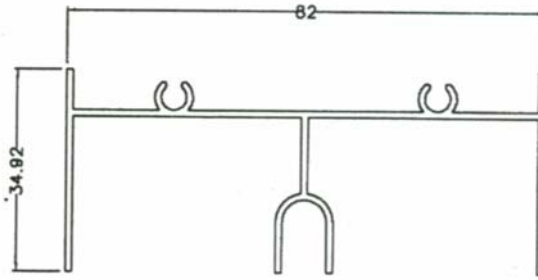
SD964 0.640 kg/m AP:430 mm
