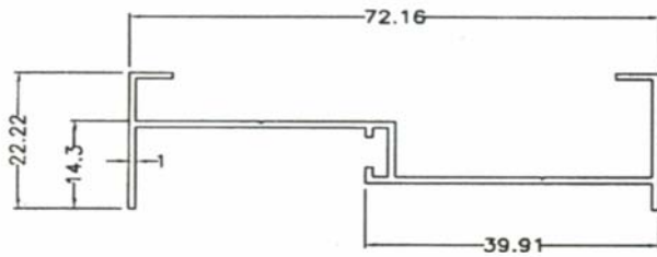
SD170 0.385 kg/m AP:282 mm
