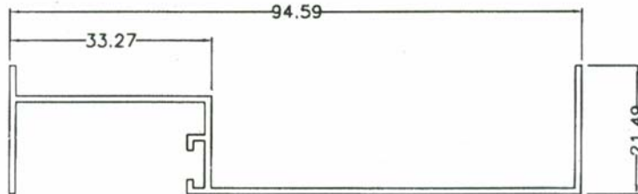
SW697N 0.461 kg/m AP: 322 mm
