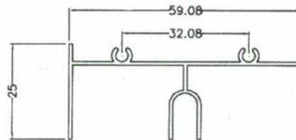
SW696 0.393 kg/m AP: 316 mm
