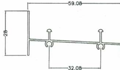
SW695 0.356 kg/m AP: 252 mm
