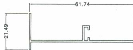
SW697 0.306 kg/m AP: 238 mm
