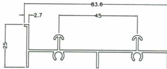
SD090 0.548 kg/m AP:366 mm
